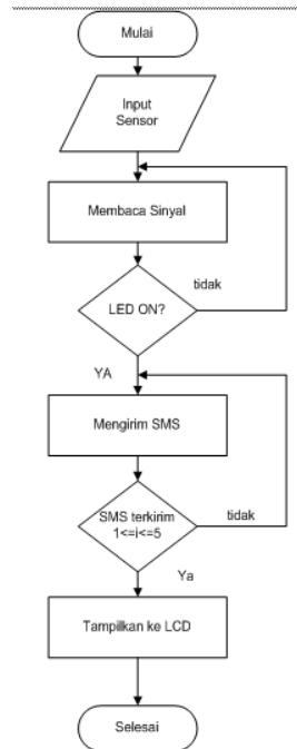
Gambar 7. Diagram Alir Sistem SMS
